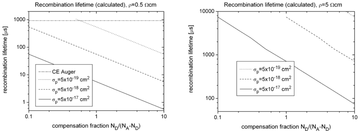
Figure 1. Bulk recombination lifetimes calculated for various capture cross sections of neutral donors. Left: 0.5 Ωcm resistivity, right: 5 Ωcm resistivity. Injection level 10^{14} \text{ cm}^{-3} , p-type silicon, donor level E_c - E_t = 0.045 eV. In the calculation of the compensation fraction, the carrier mobilities are assumed to be unchanged by the compensation. In reality the lines would probably not be straight due to dopant-dopant-interaction.
